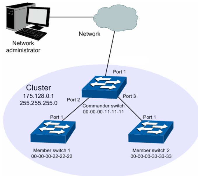
Figure 14-19 Network diagram
