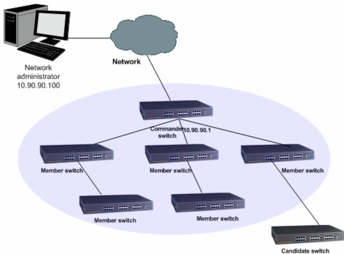
Figure 14-1 Cluster topology
